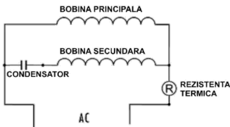
DIAGRAMA ELECTRICA
